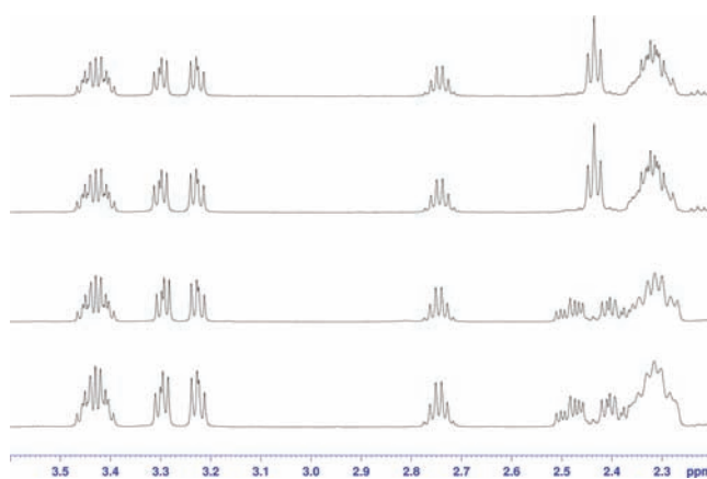
Figure 5. Partial ^1\text{H} NMR spectra (600 MHz, \text{CDCl}_3 ) of ( 3S,7S,11R,15R )- 20a,b , ( 3S,7S,11R,15S )- 20a,c , ( 3R,7S,11R,15R )- 20b,b , and ( 3R,7S,11R,15S )- 20b,c (top to bottom). Most parts of the spectra are very similar, but notice the differences in the region 2.4–2.5 ppm.
